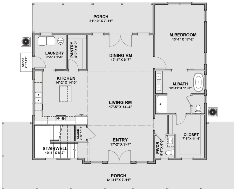
Main Floor
